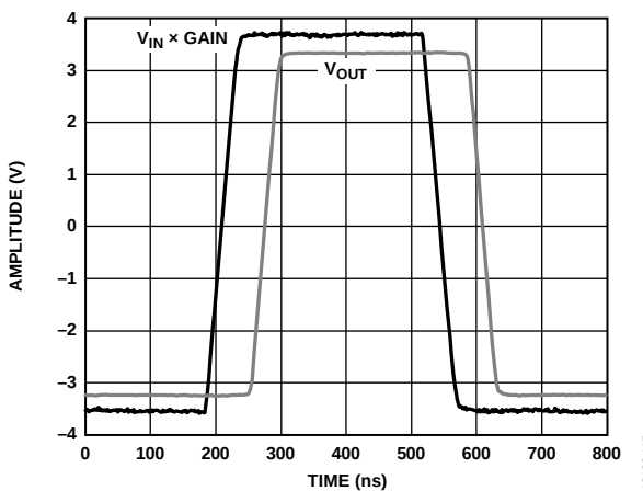
Figure 14. Overdrive Recovery
