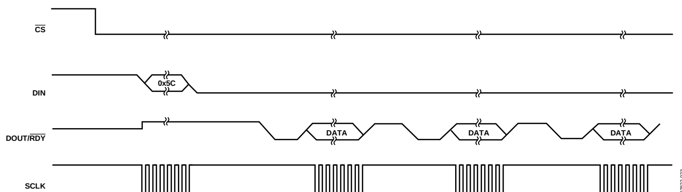
Figure 31. Continuous Read
