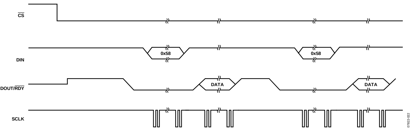
Figure 30. Continuous Conversion
