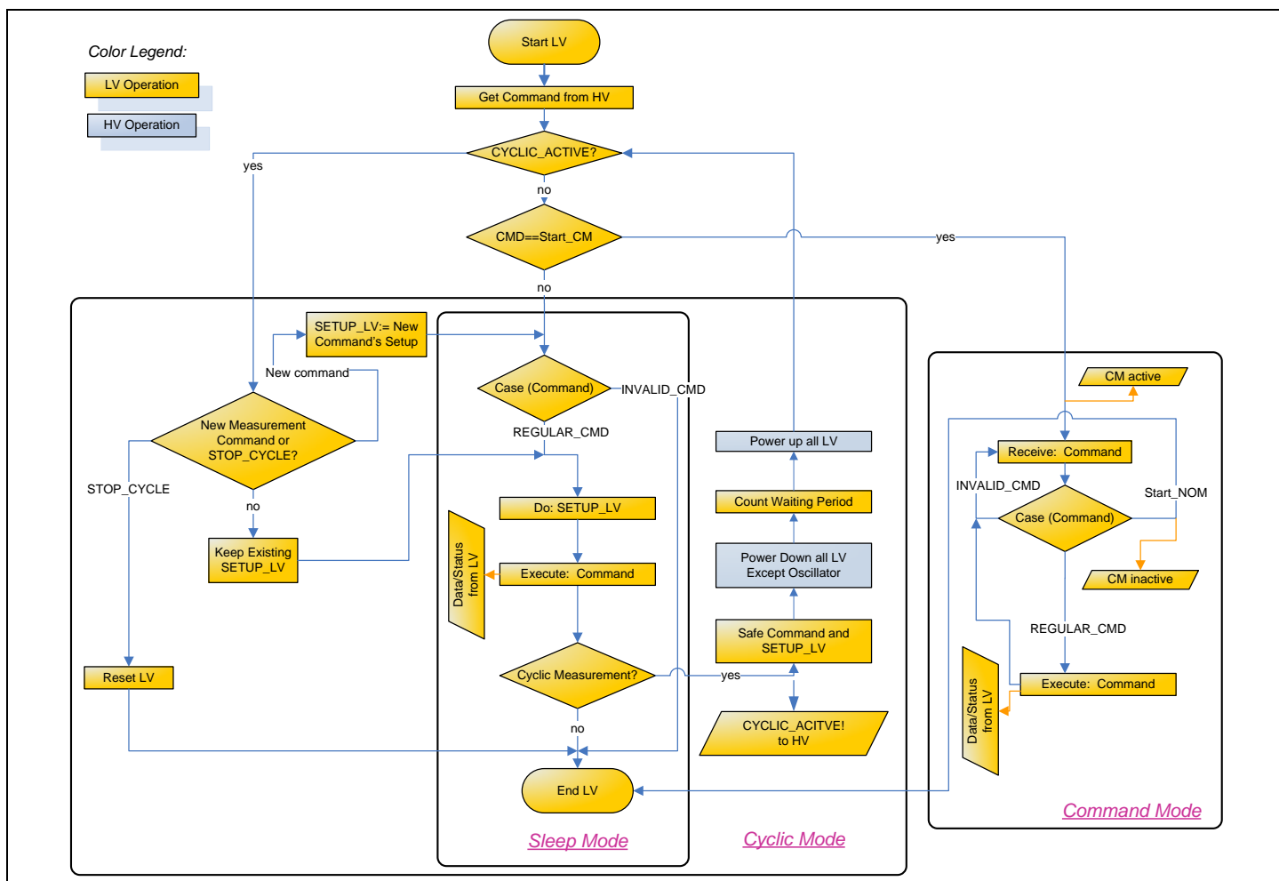
Figure 3.3 Operational Flow Chart: Command Mode and Normal Mode (Sleep and Cyclic)
