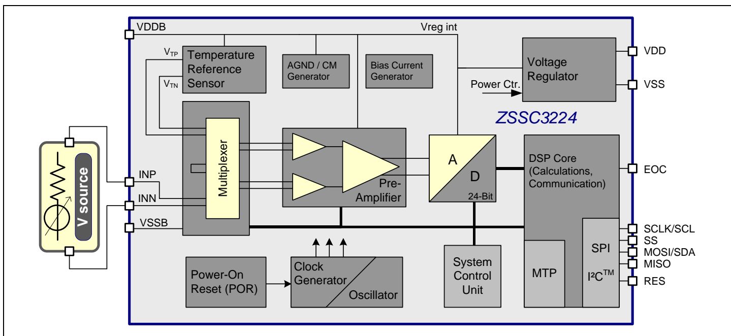
Figure 2.2 ZSSC3224 Functional Block Diagram with Voltage-Source Sensor
