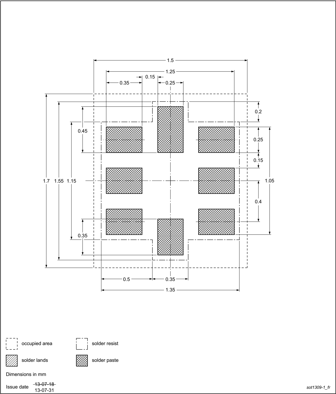
Footprint information for reflow soldering of SOT1309 package SOT1309-1
