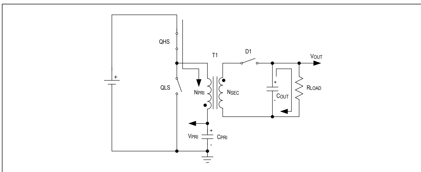
Figure 2. On Period Equivalent Circuit
