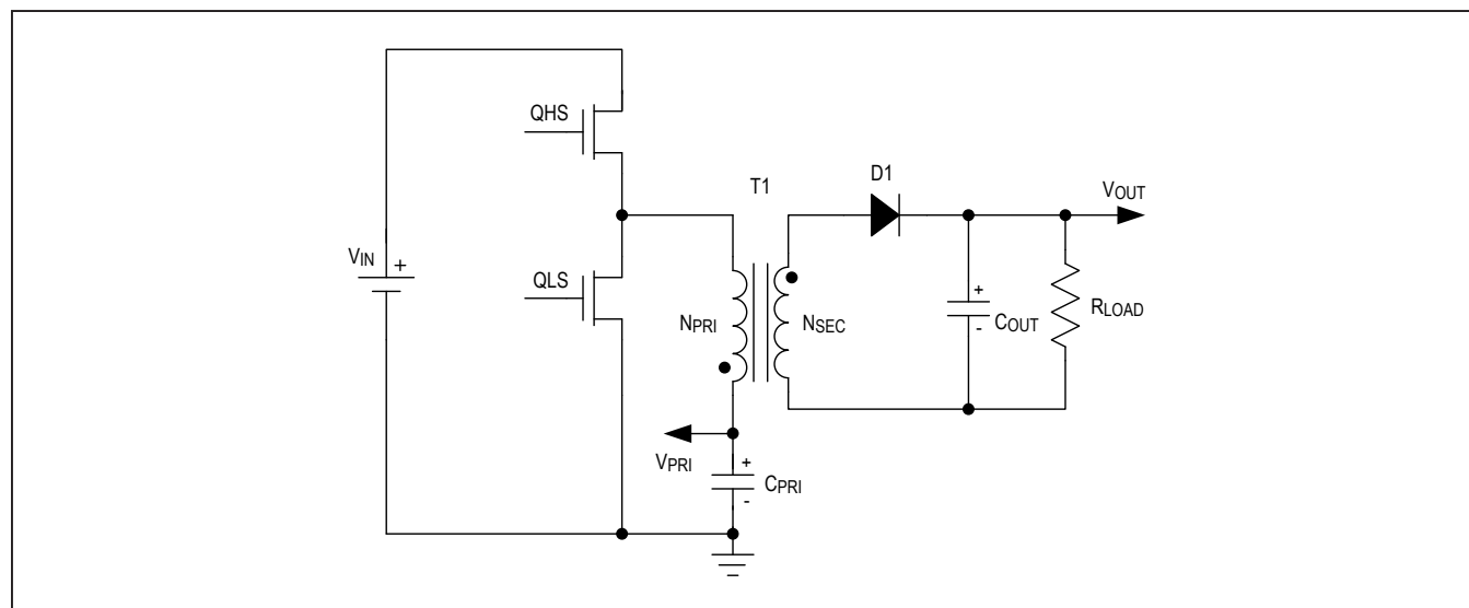
Figure 1. Iso-Buck Topology
